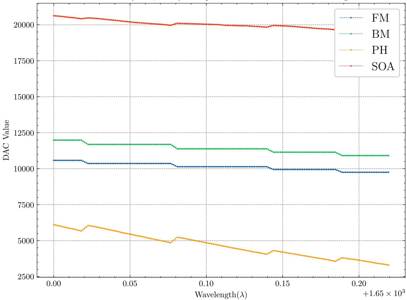
DAC Parameters (5000, 5050) Interpolated with 3 Intermediate Integer Values
